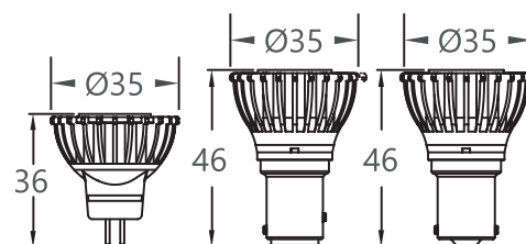
Base Type : GU4.0 BA15D BA15S
